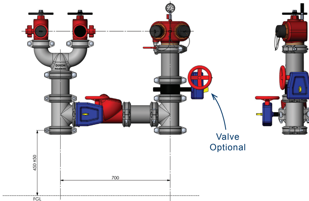
100NB Assembly
