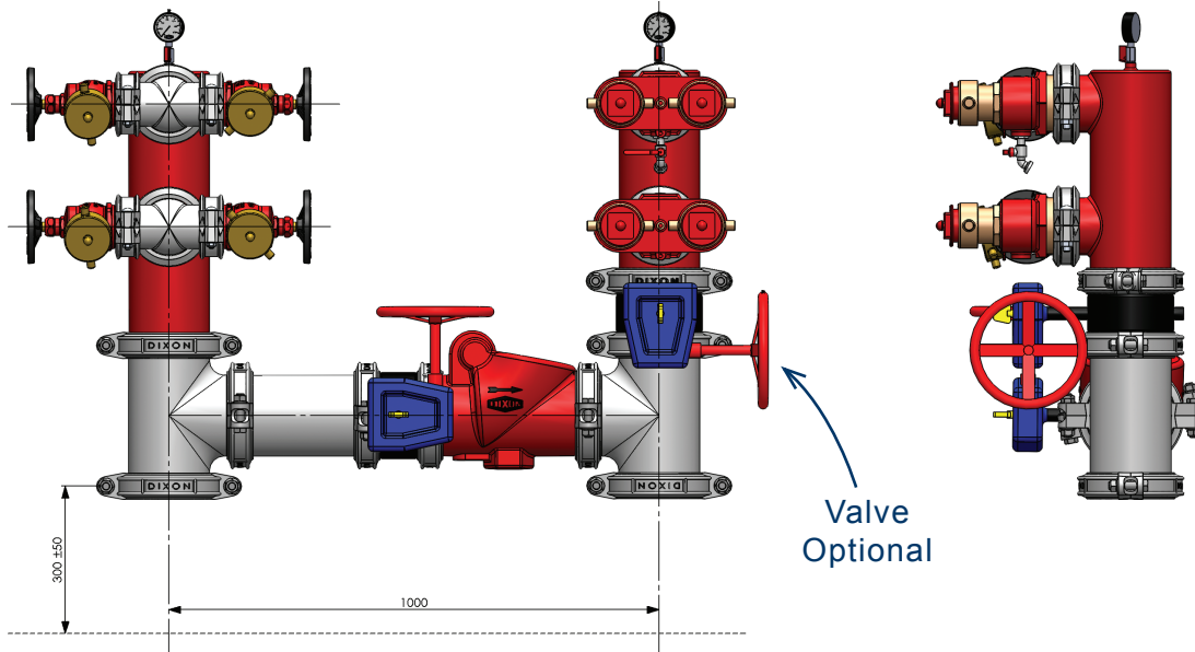
150NB & 200NB Assembly
