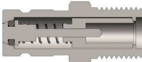
Male Thread
