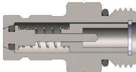
Male ORB Thread
