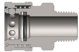
Male Thread
