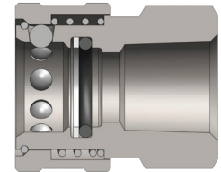
Female Thread
