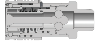
Male Thread
